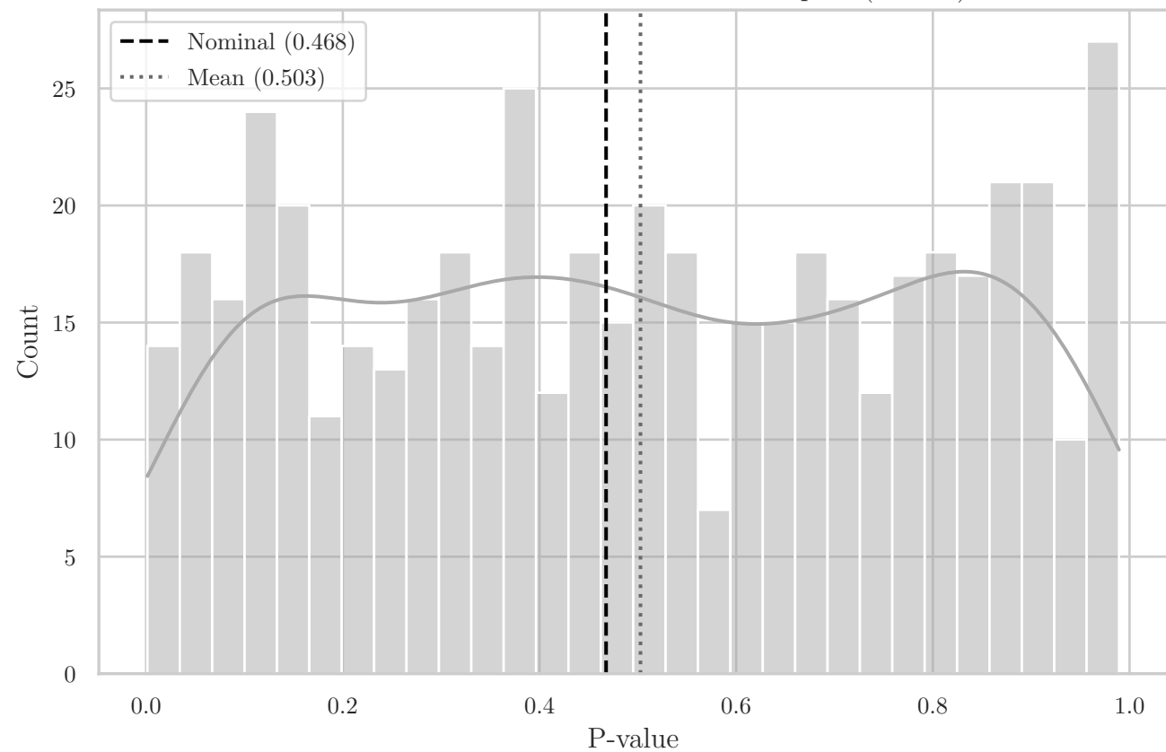
MC Distribution of P-values for ST Compact (F2 XY)
