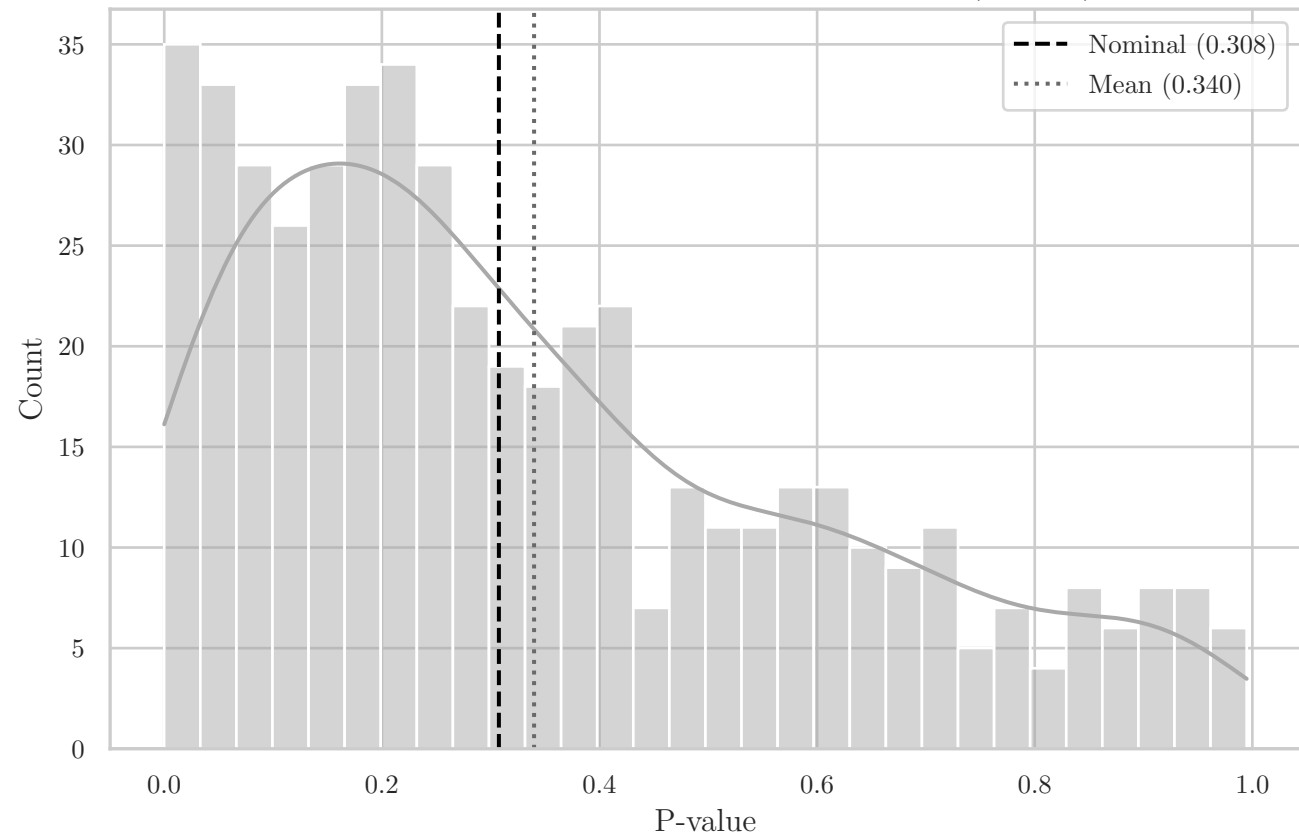
MC Distribution of P-values for QRS Compact (OO YZ)
