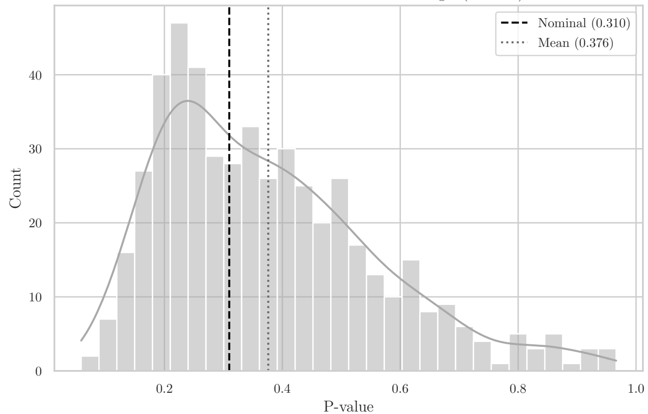
MC Distribution of P-values for ST Angle (OO YZ)
