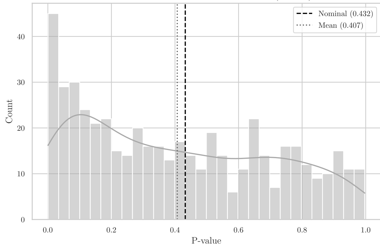
MC Distribution of P-values for ST T-Dist (OO YZ)
