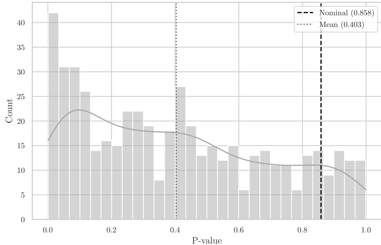
MC Distribution of P-values for ST T-Dist (OQ XY)
