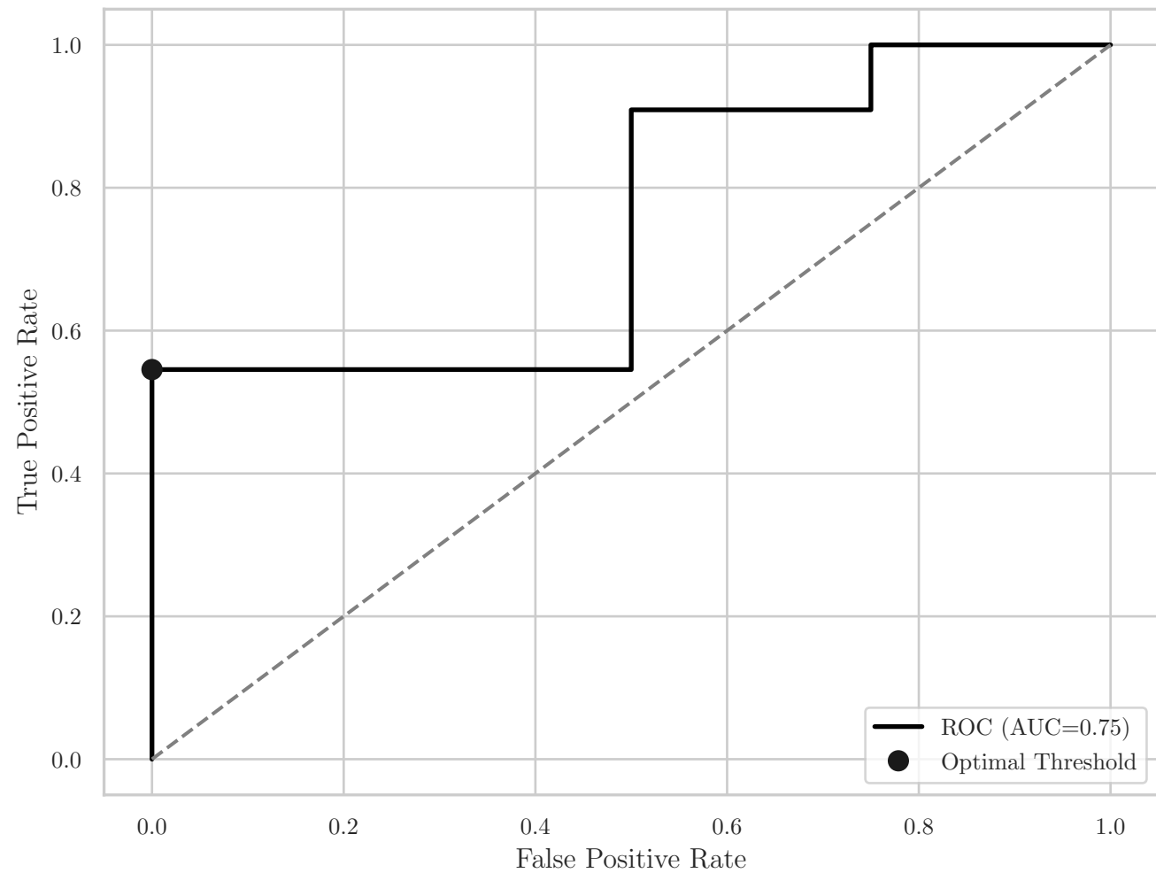
ROC Curve
