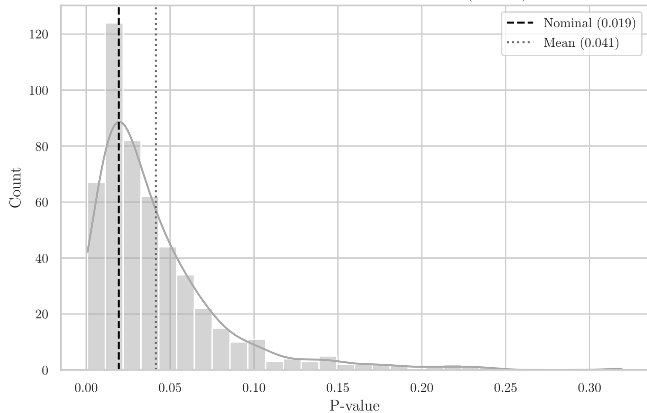
MC Distribution of P-values for T T-Dist (OT YZ)
