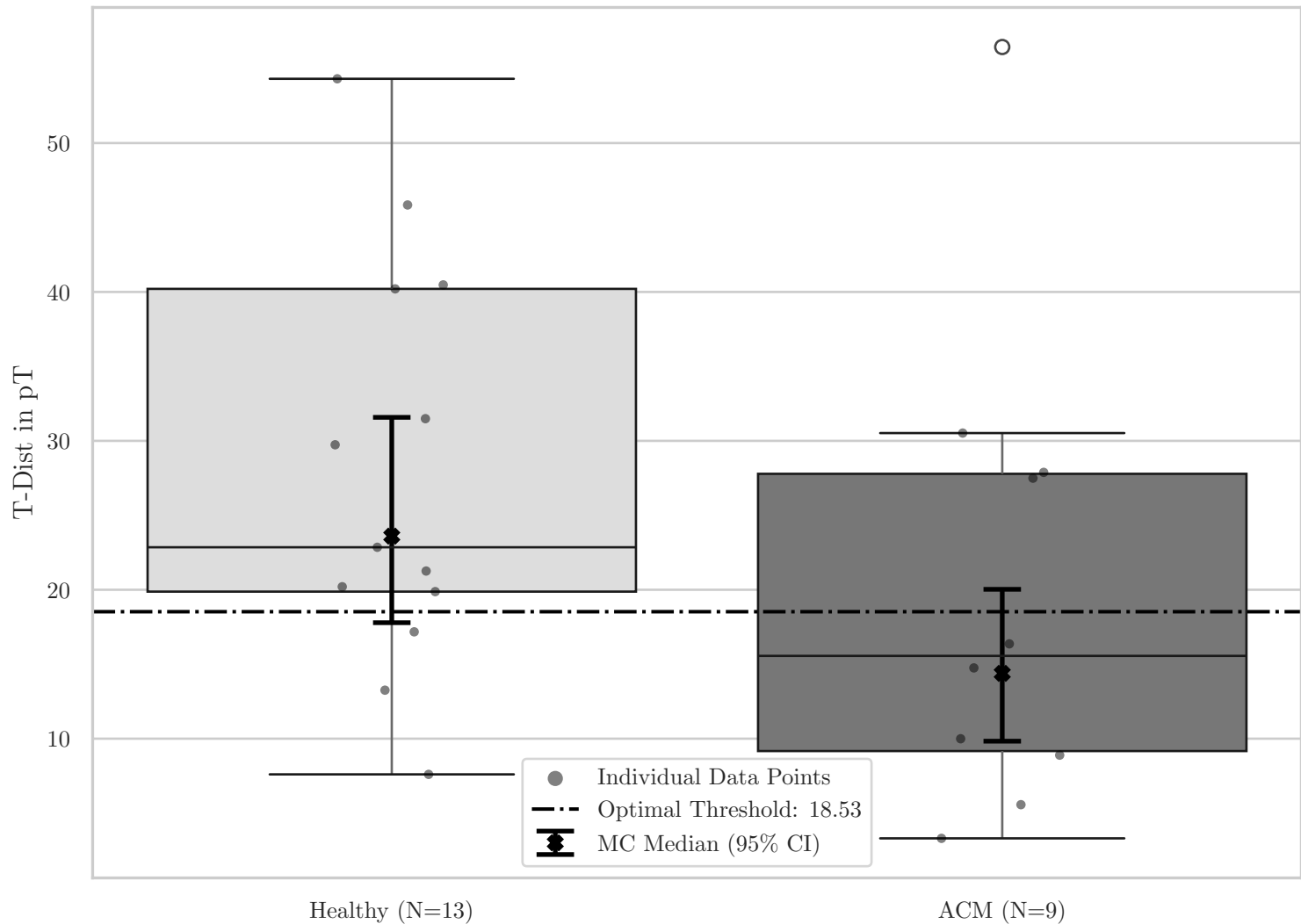
Box Plot for QRS T-Dist (OY XY)
