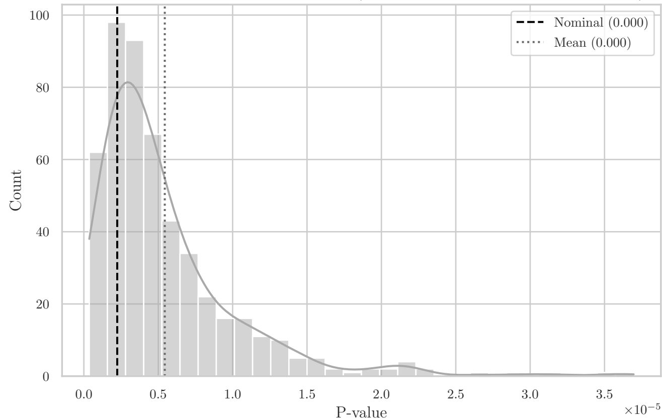
MC Distribution of P-values for T Area (Aggregated Bottom-Right Quadrant YZ)
