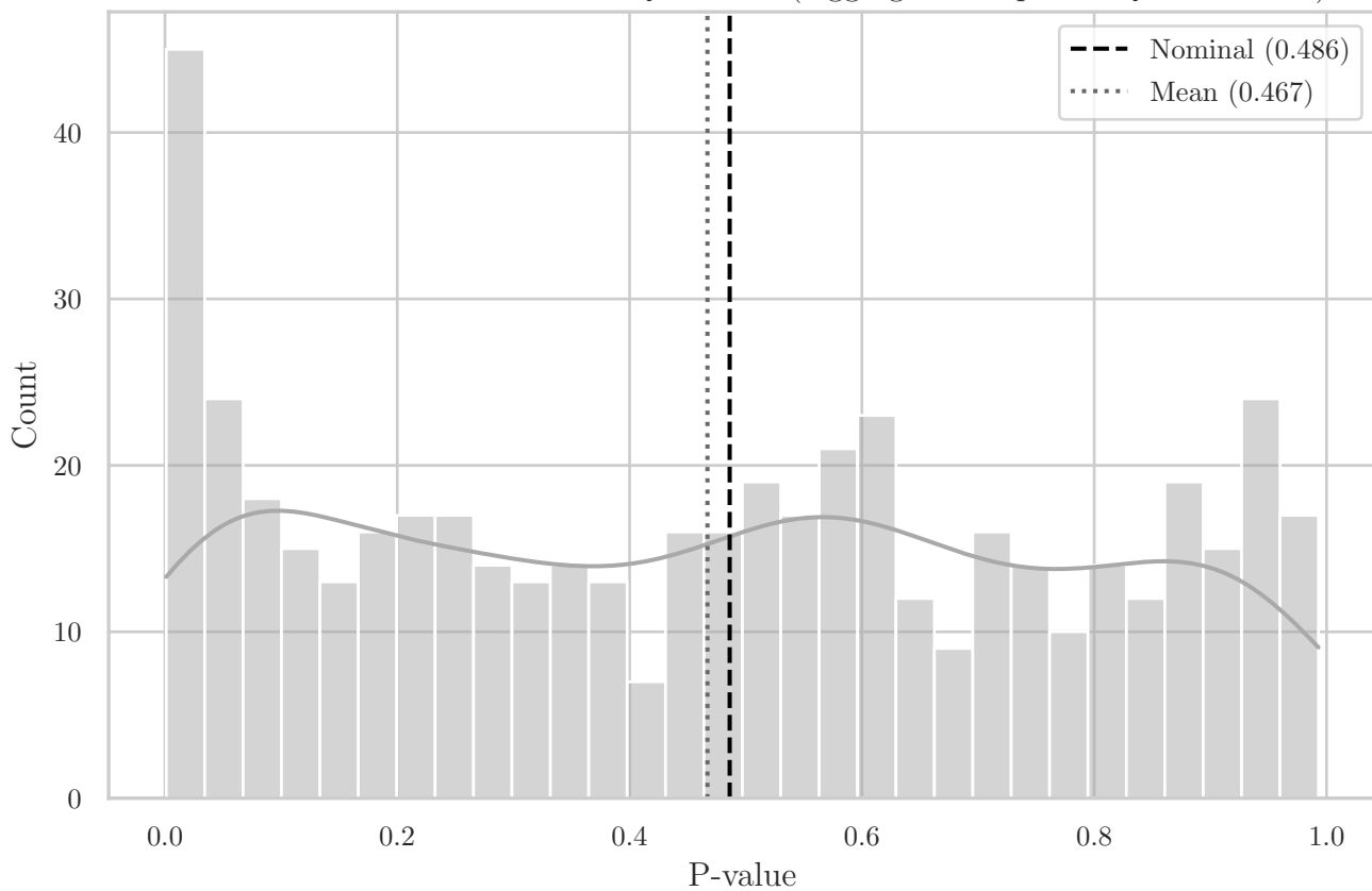
MC Distribution of P-values for QRS Area (Aggregated Top-Left Quadrant XY)
