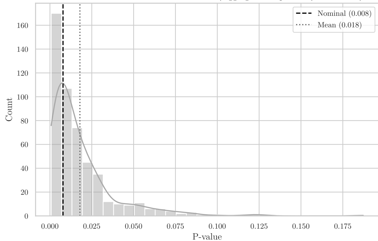
MC Distribution of P-values for T T-Dist (Aggregated Top-Left Quadrant YZ)
