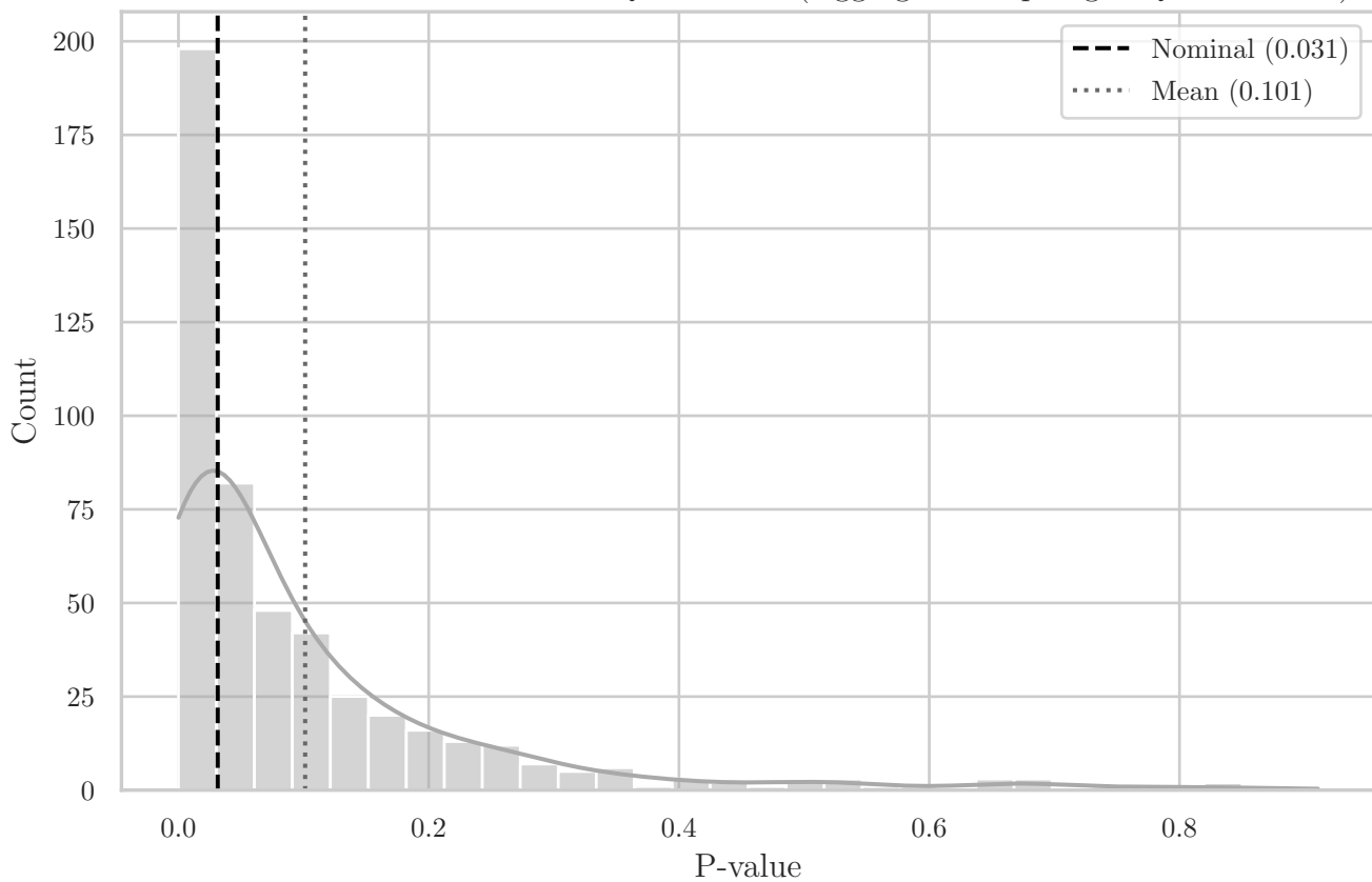
MC Distribution of P-values for QRS T-Dist (Aggregated Top-Right Quadrant XY)
