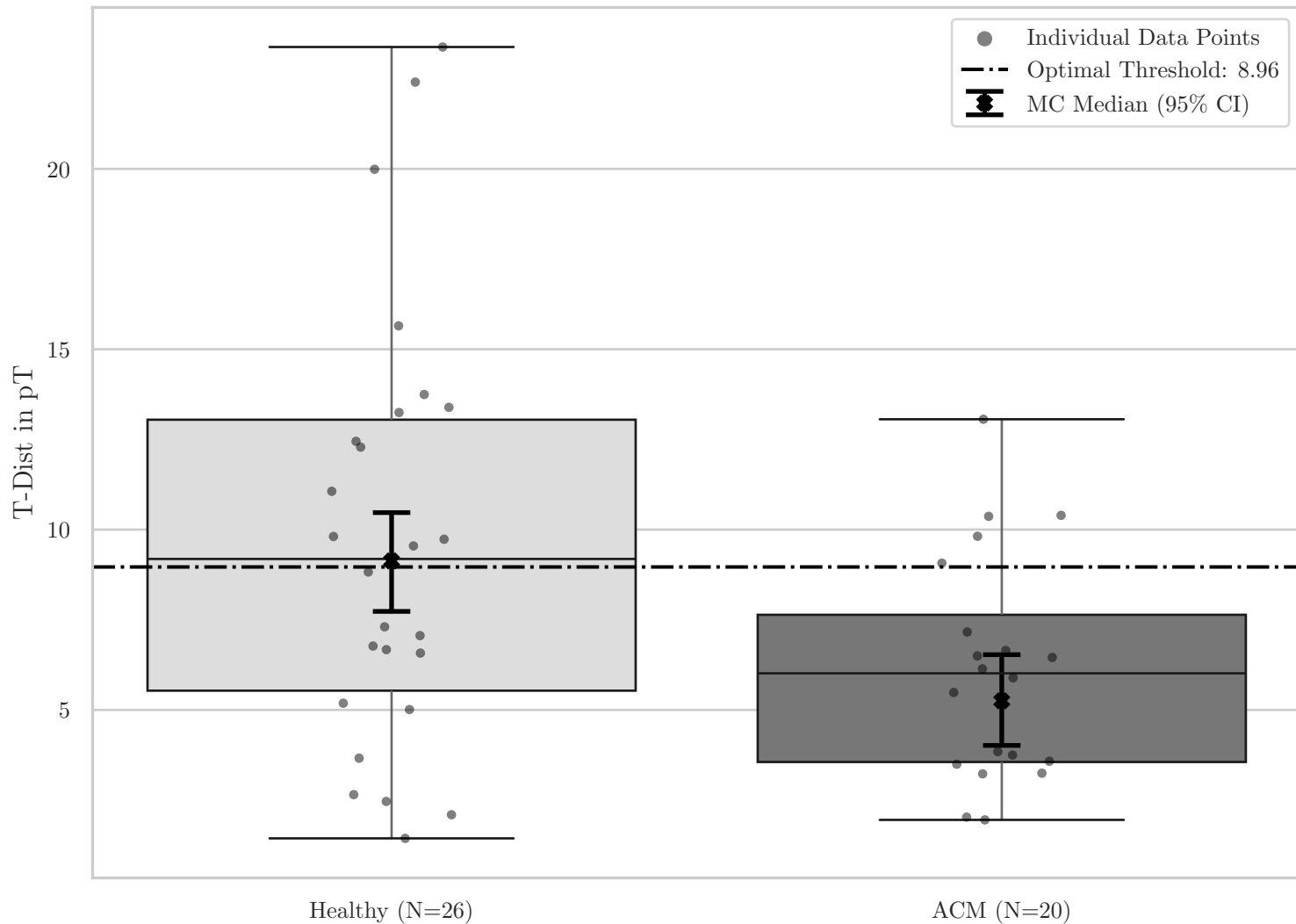
Box Plot for T T-Dist (Aggregated Top-Right Quadrant XY)
