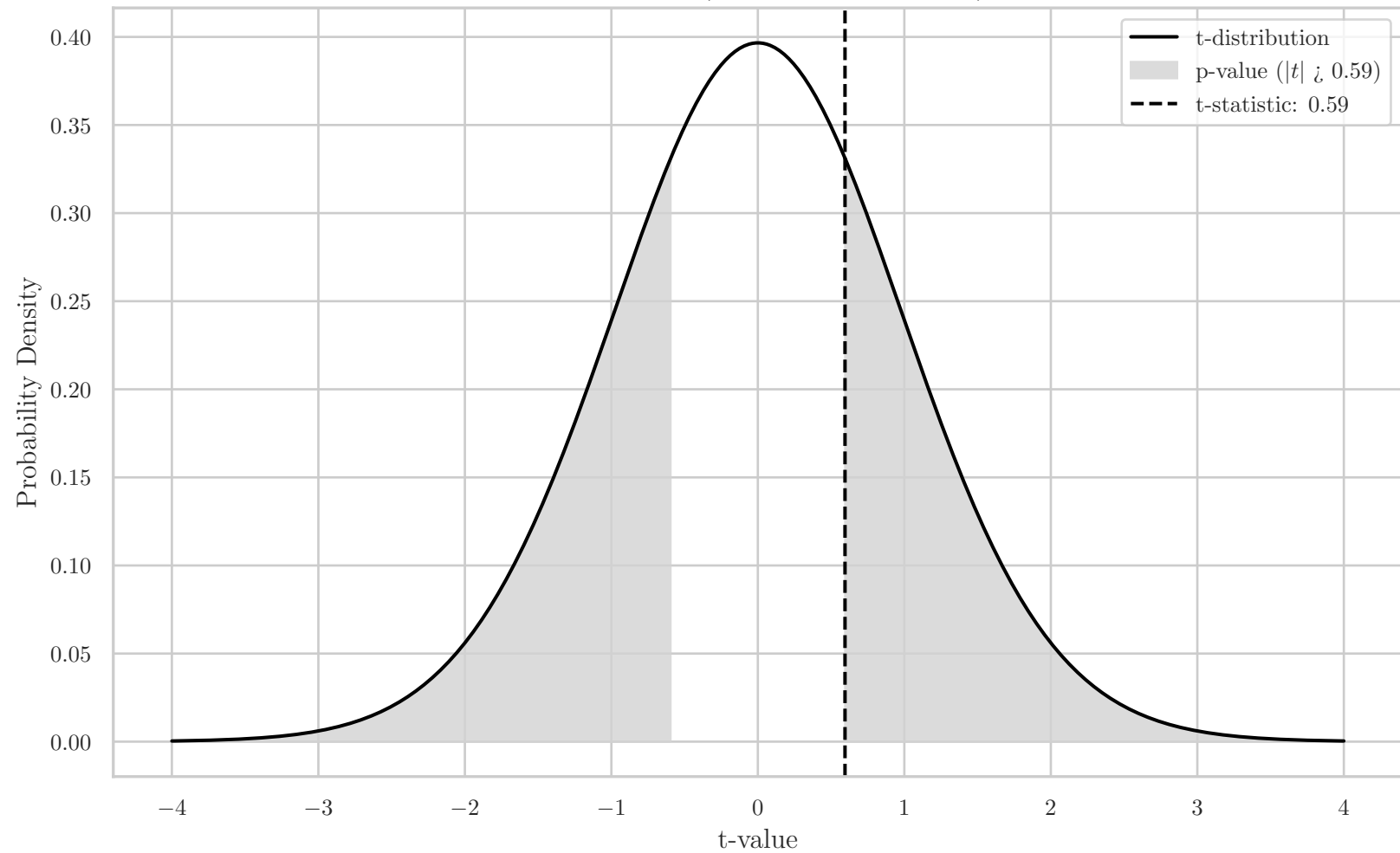
t-Distribution (Hyp: Healthy \neq ACM)
