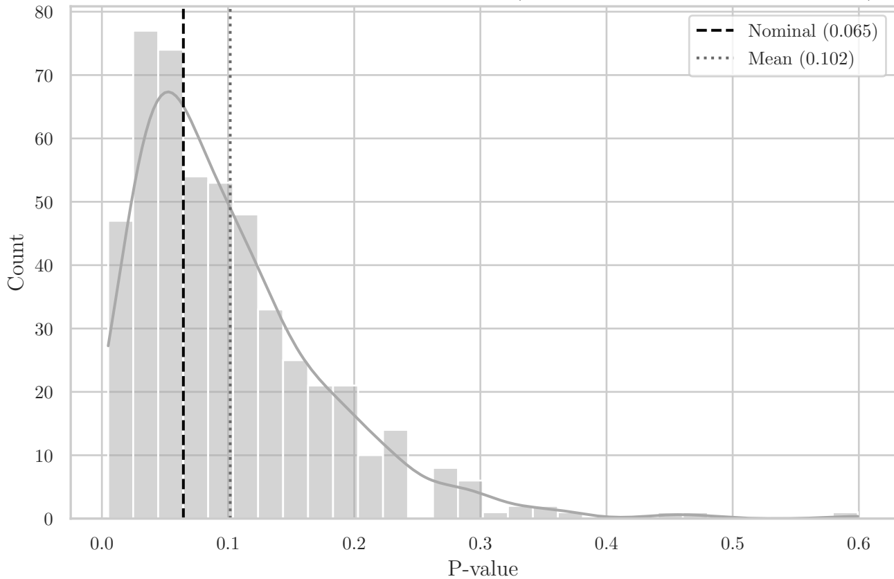
MC Distribution of P-values for T Compact (Aggregated Top-Right Quadrant YZ)
