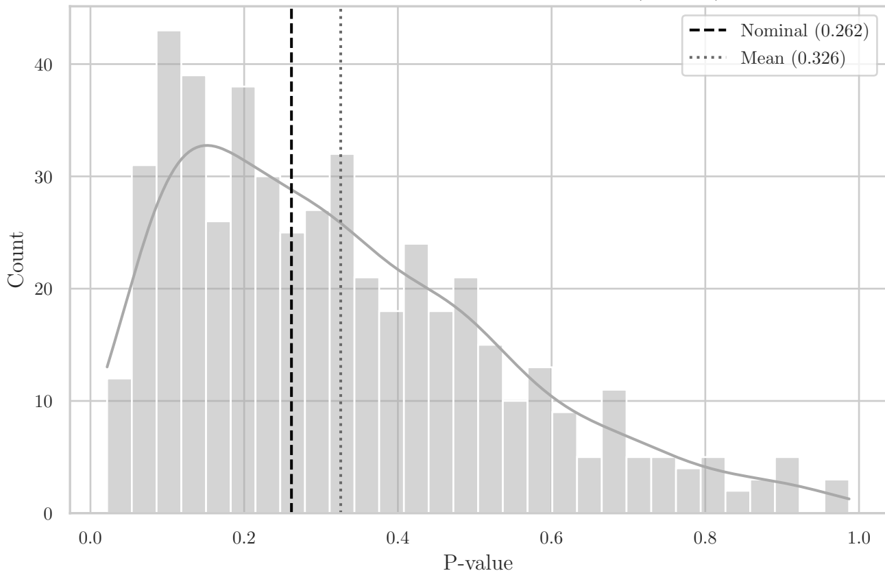
MC Distribution of P-values for ST Angle (YQ XY)
