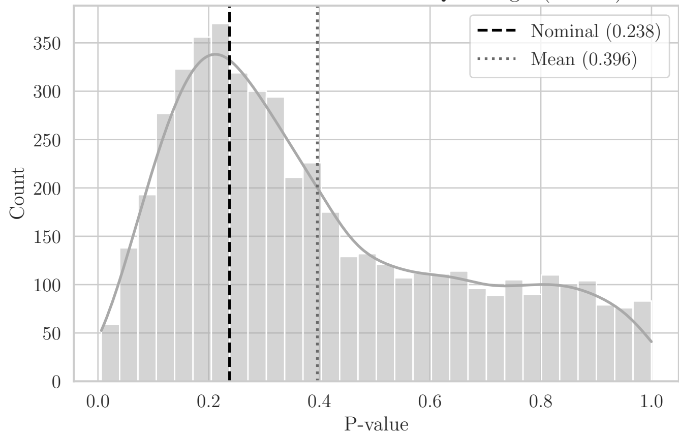
MC Distribution of P-values for QRS Angle (C1 XY)
