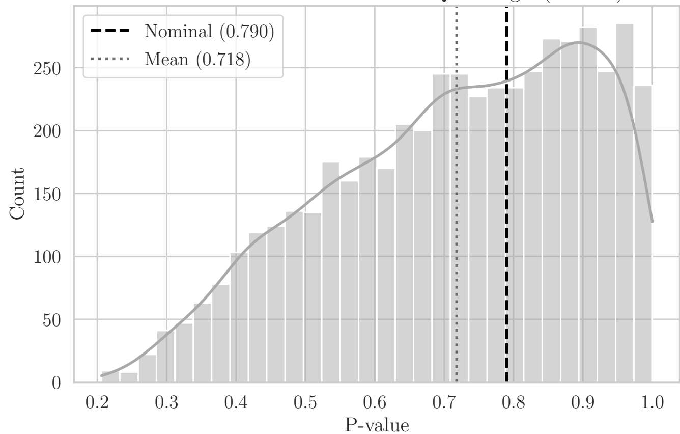
MC Distribution of P-values for QRS Angle (NL YZ)
