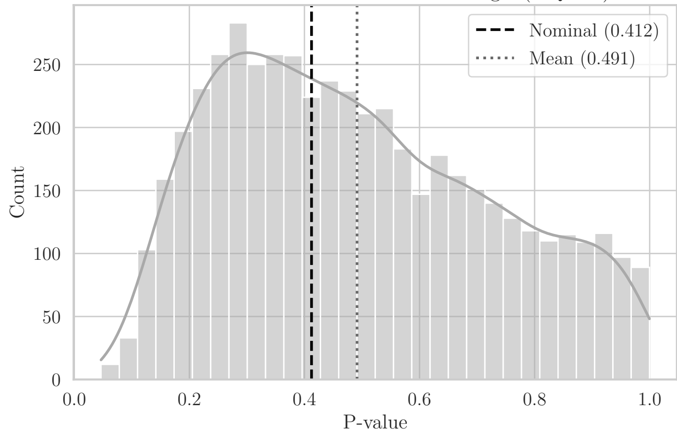
MC Distribution of P-values for T Angle (OQ XY)
