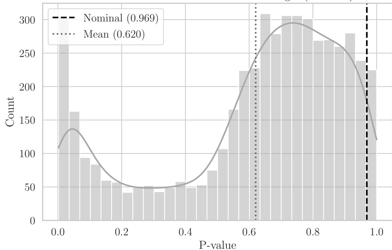
MC Distribution of P-values for T Angle (OR XY)
