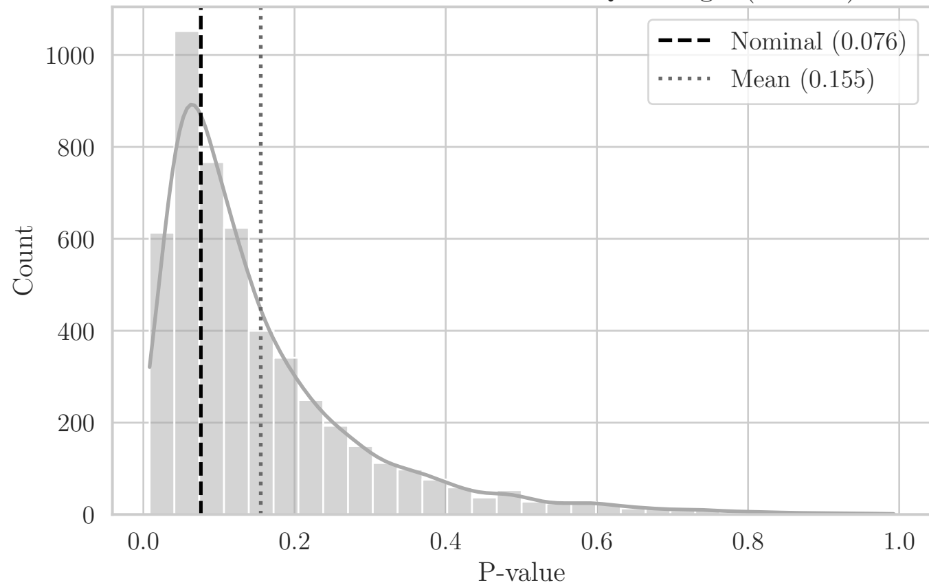
MC Distribution of P-values for QRS Angle (OT YZ)
