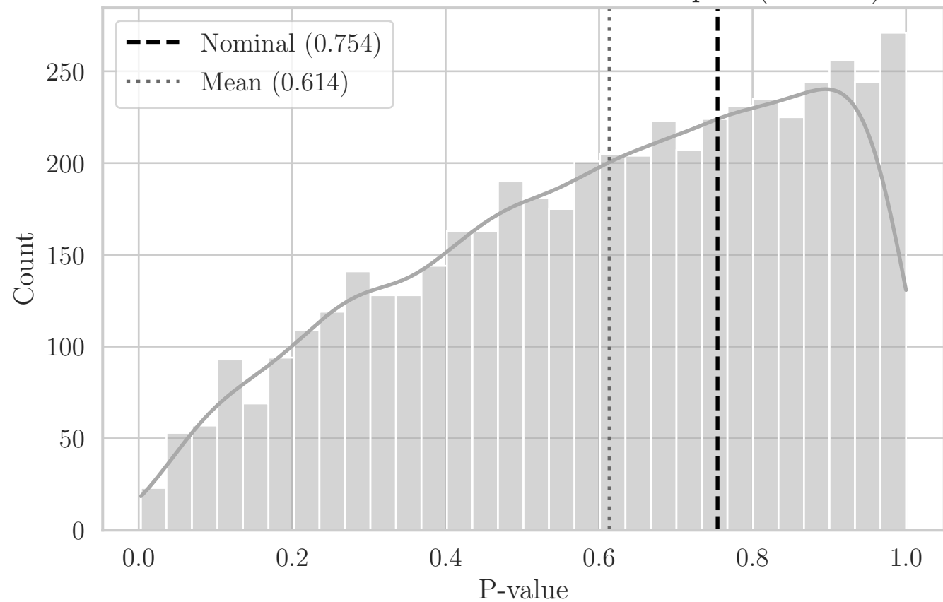
MC Distribution of P-values for ST Compact (OW YZ)
