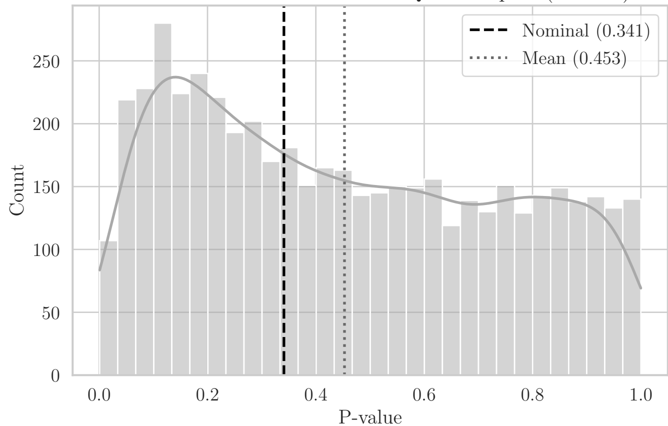
MC Distribution of P-values for QRS Compact (OX XY)
