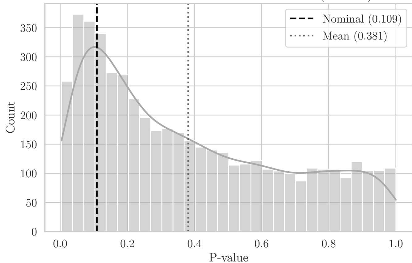
MC Distribution of P-values for ST Area (OY XY)
