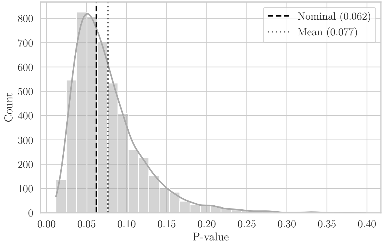
MC Distribution of P-values for T Angle (Aggregated Bottom-Left Quadrant YZ)
