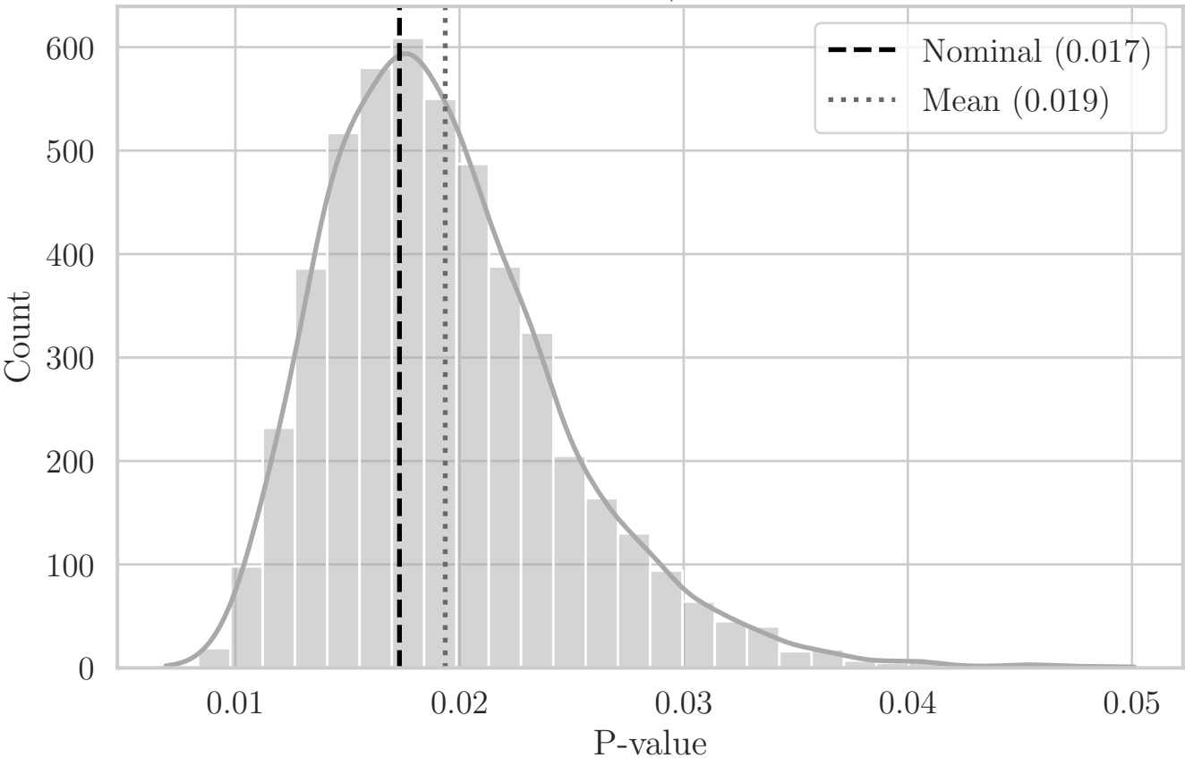
MC Distribution of P-values for QRS Area (Aggregated Bottom-Right Quadrant XY)
