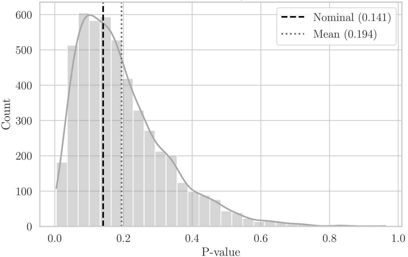
MC Distribution of P-values for T Compact (Aggregated Top-Right Quadrant XY)
