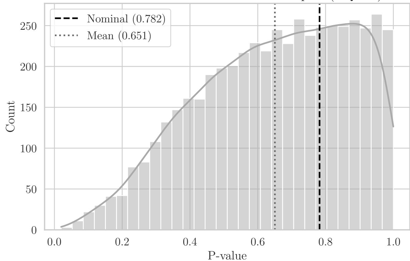
MC Distribution of P-values for ST Compact (YQ XY)
