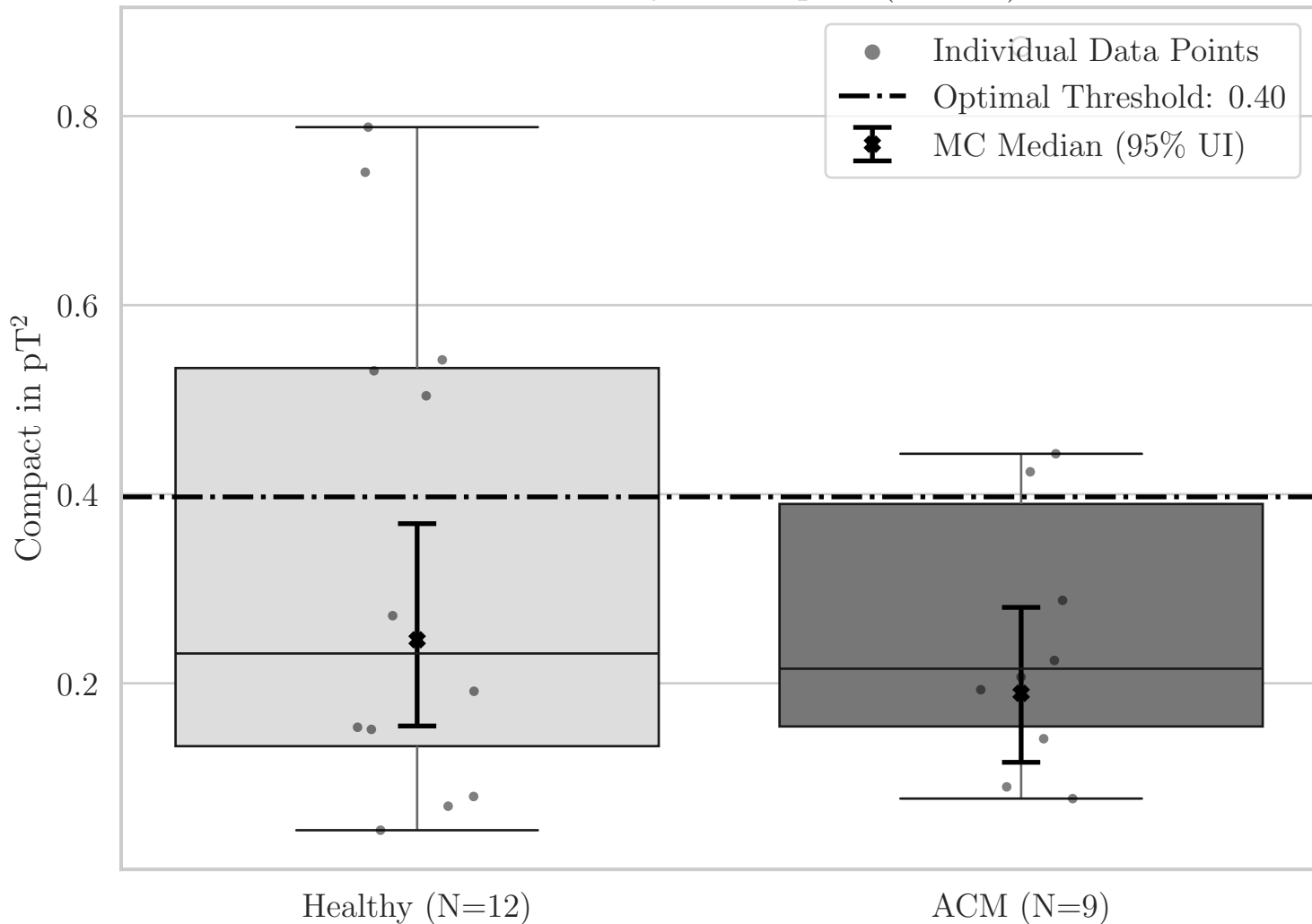
Box Plot for QRS Compact (EZ YZ)
