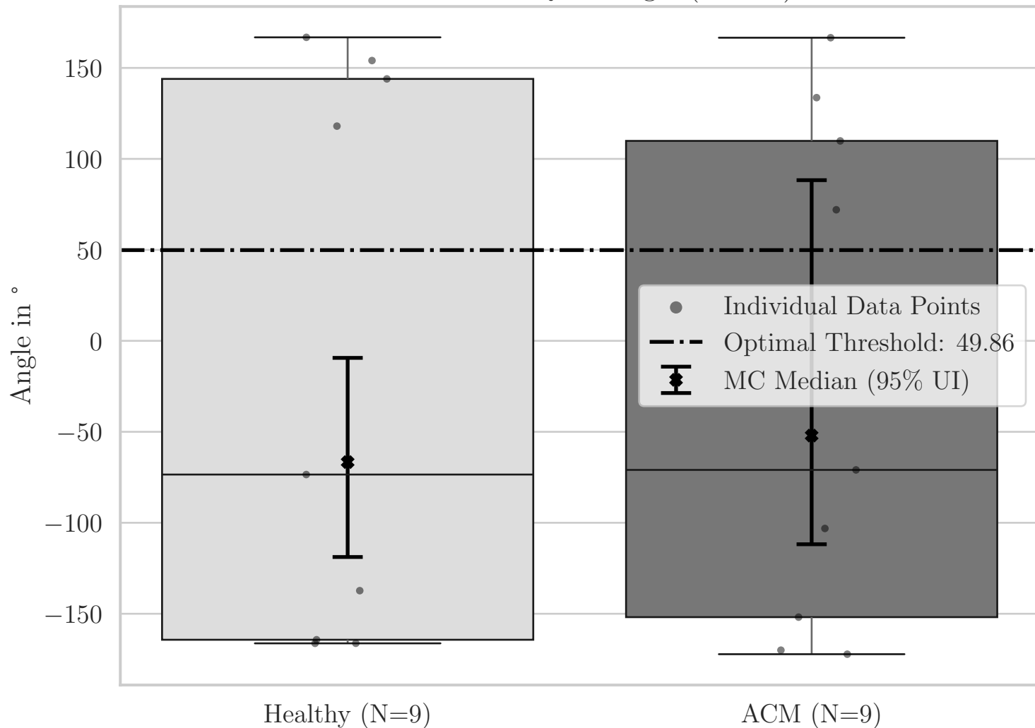
Box Plot for QRS Angle (F0 YZ)
