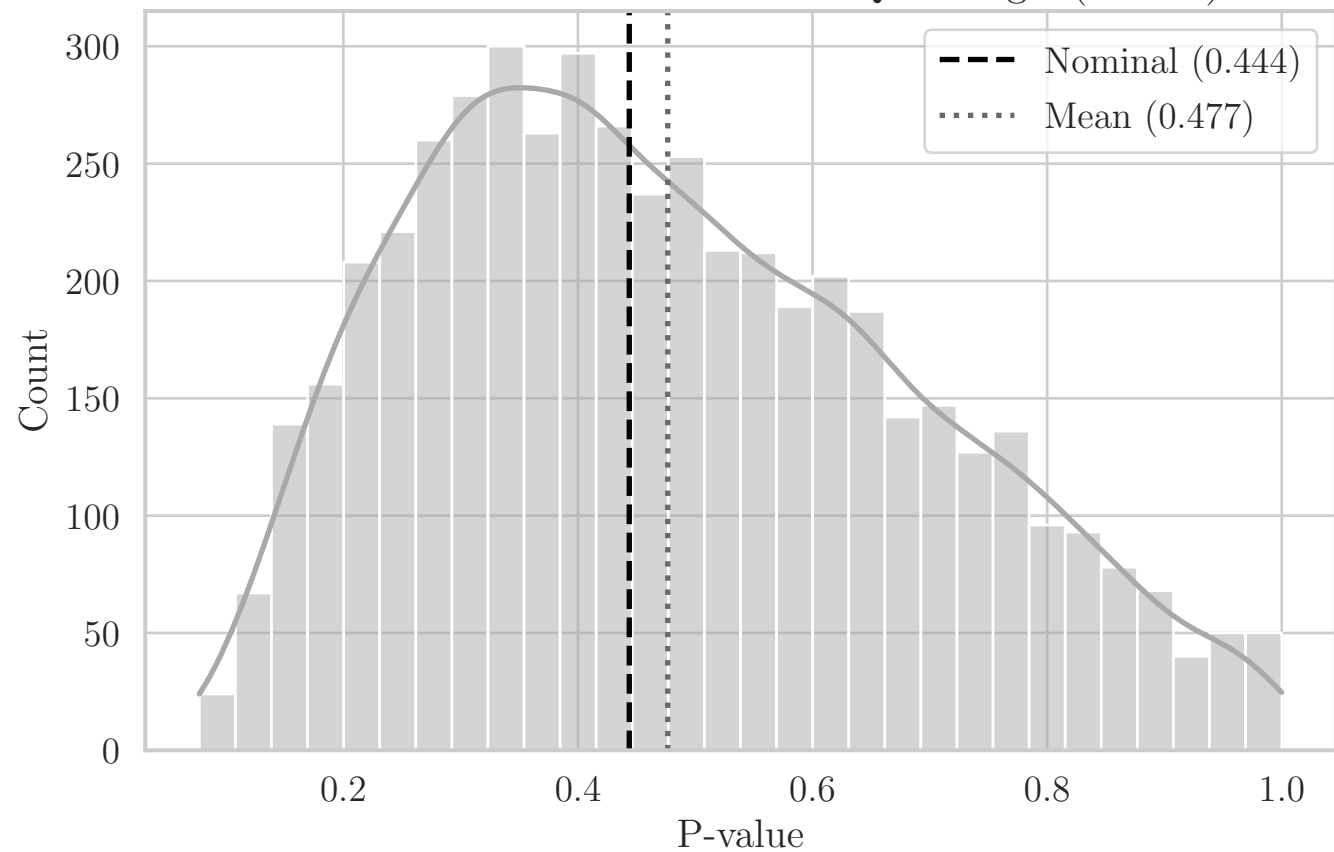
MC Distribution of P-values for QRS Angle (F1 YZ)
