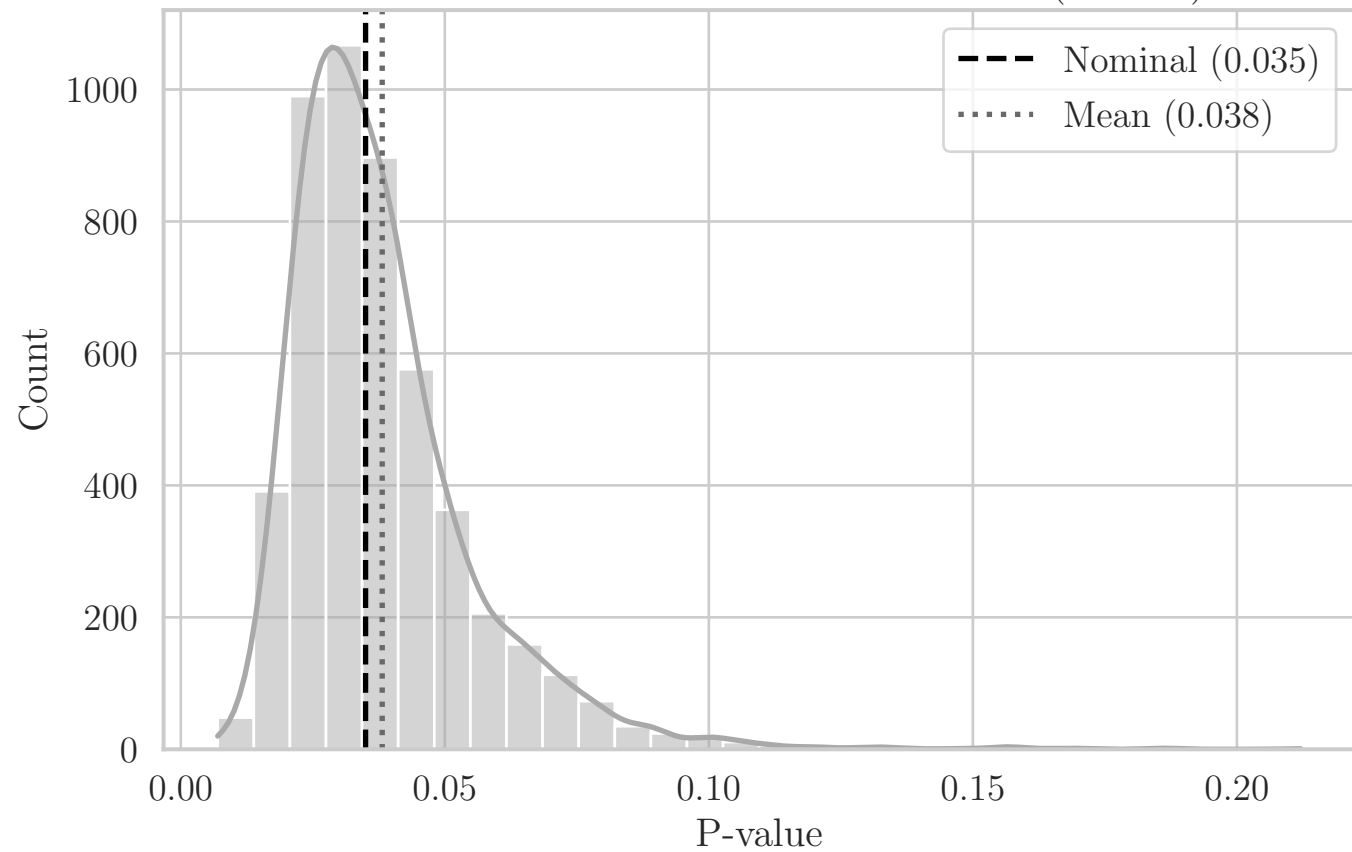
MC Distribution of P-values for T Area (F2 XY)
