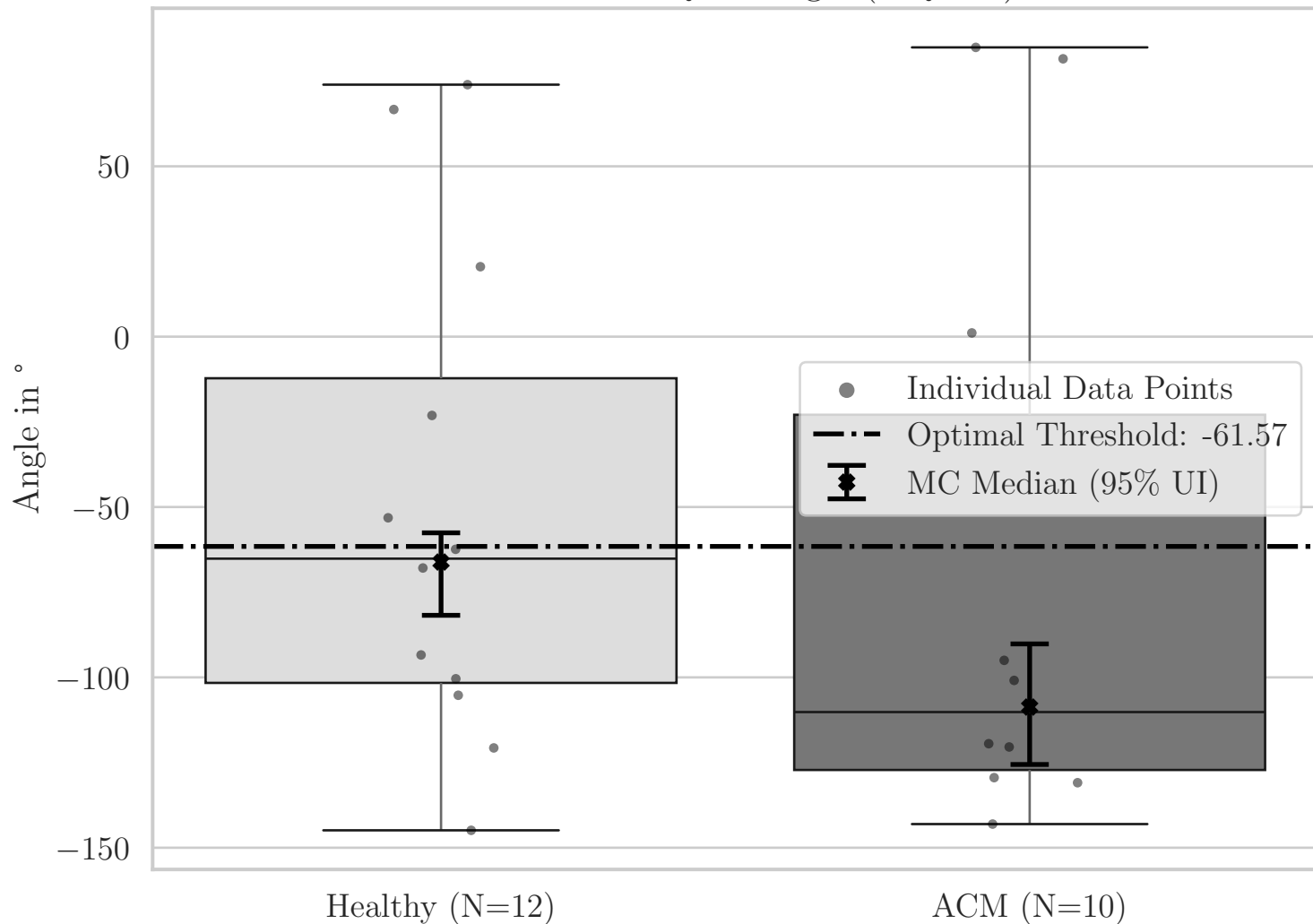
Box Plot for QRS Angle (OQ XY)
