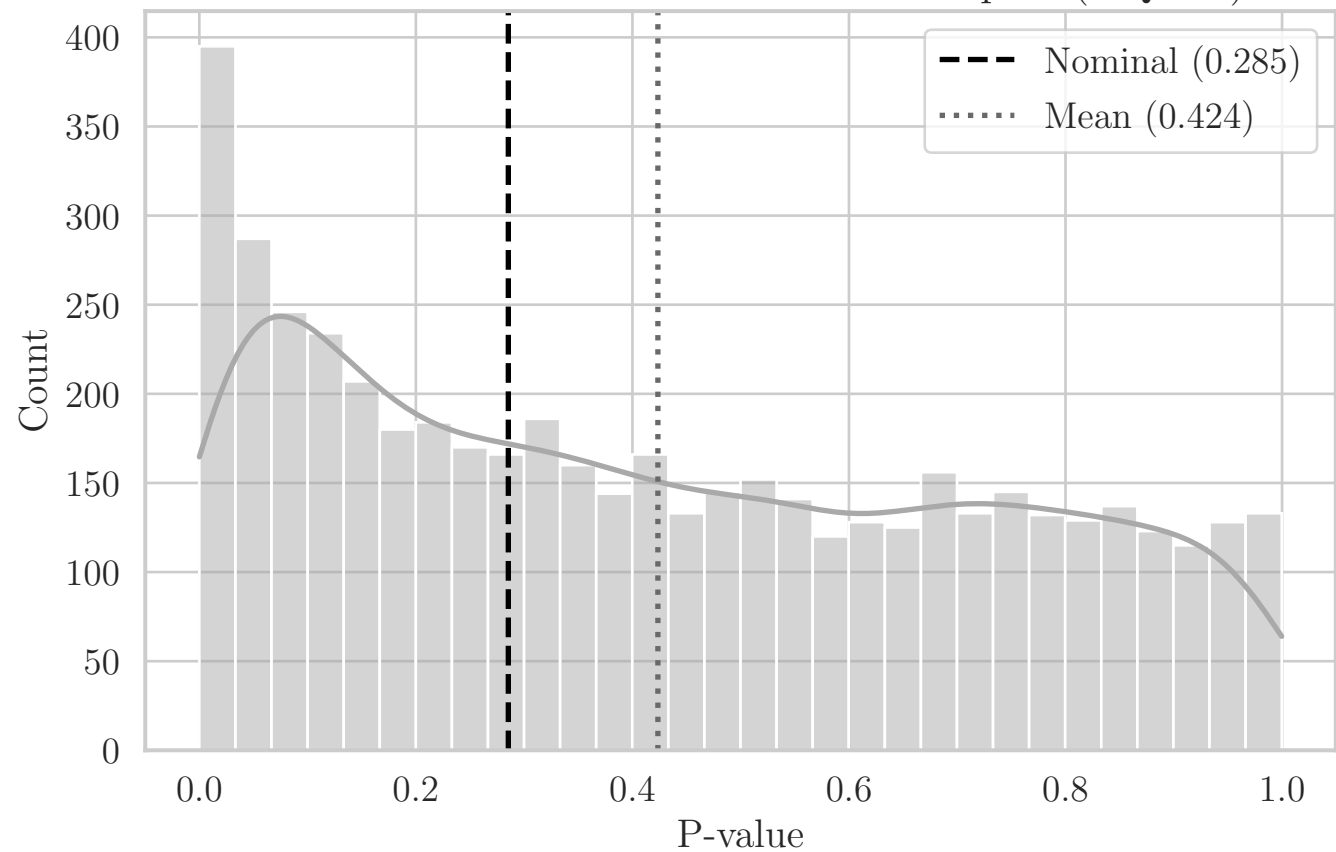
MC Distribution of P-values for ST Compact (OQ XY)
