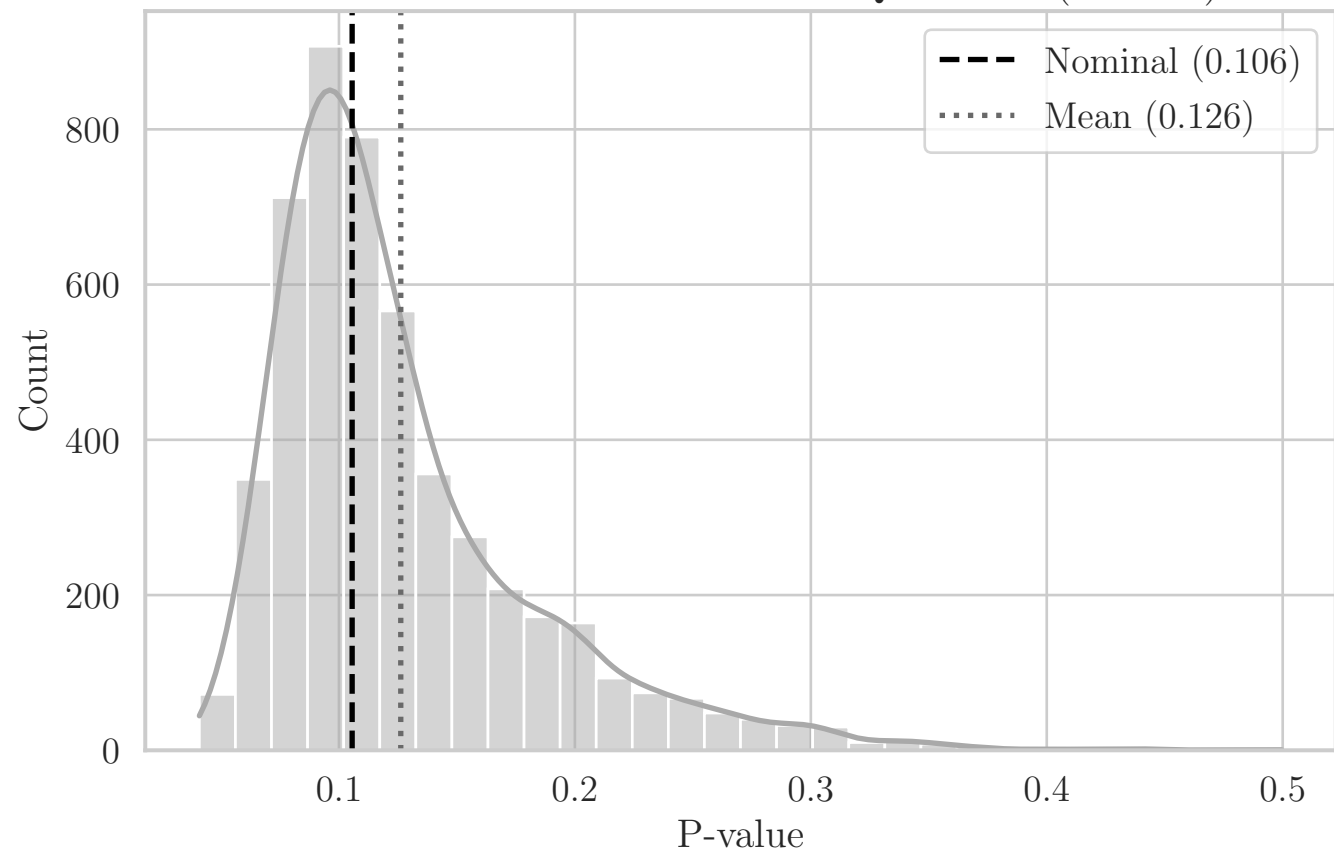
MC Distribution of P-values for QRS Area (OT YZ)
