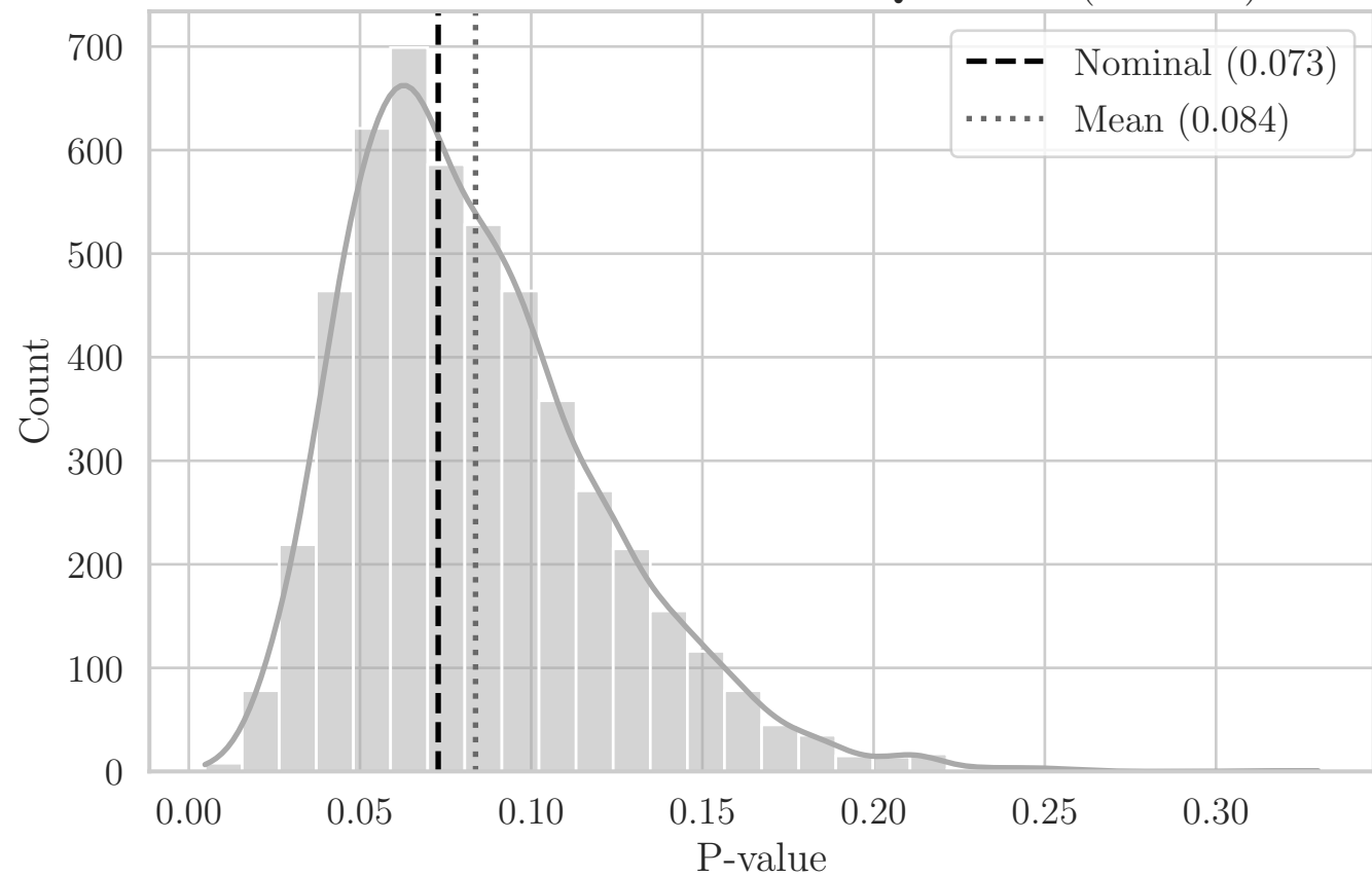
MC Distribution of P-values for QRS Area (OW YZ)
