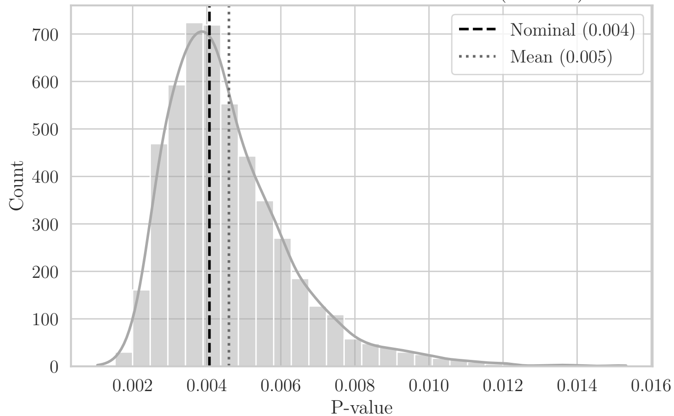
MC Distribution of P-values for T Area (OW YZ)
