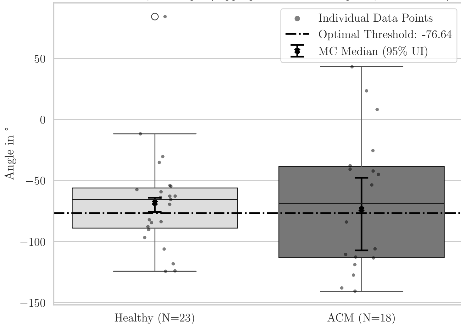
Box Plot for QRS Angle (Aggregated Bottom-Right Quadrant XY)
