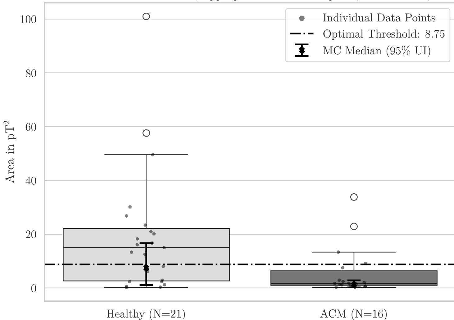
Box Plot for ST Area (Aggregated Bottom-Right Quadrant XY)
