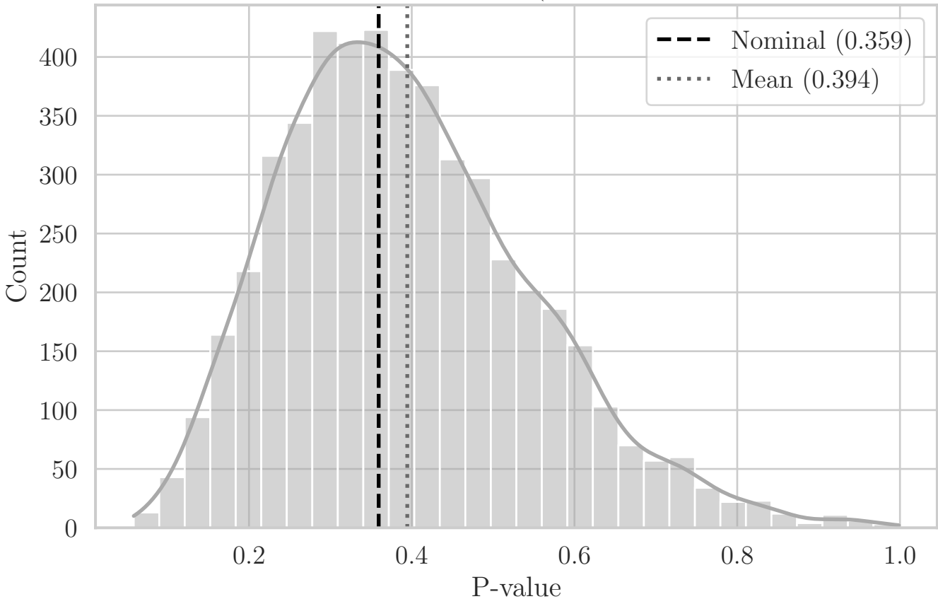
MC Distribution of P-values for T Compact (Aggregated Bottom-Right Quadrant YZ)
