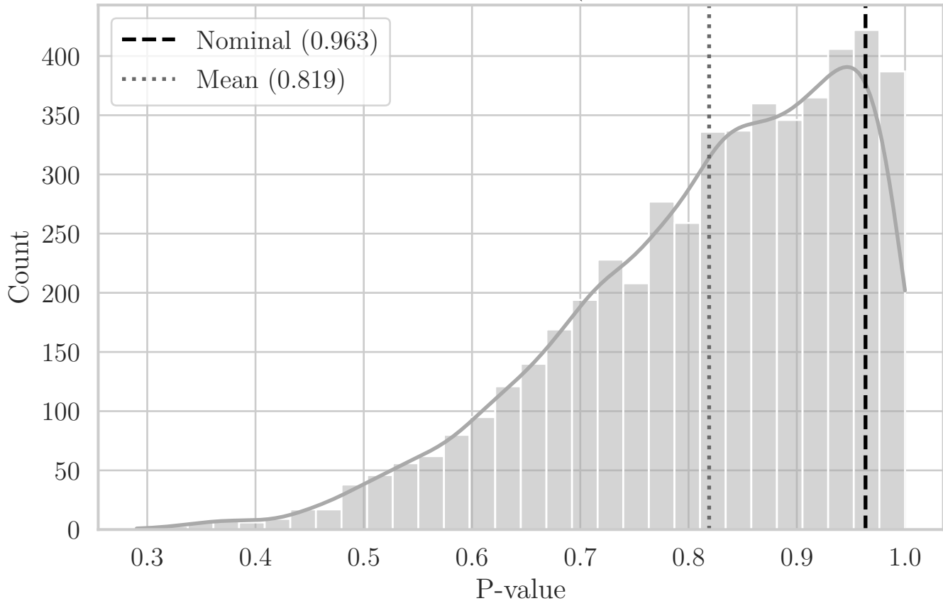
MC Distribution of P-values for T Compact (Aggregated Top-Left Quadrant YZ)
