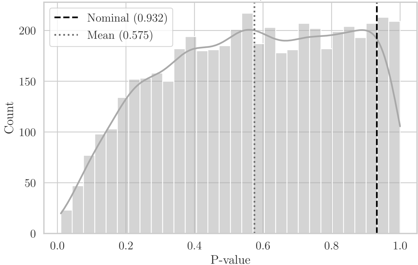
MC Distribution of P-values for QRS Compact (Aggregated Top-Right Quadrant XY)
