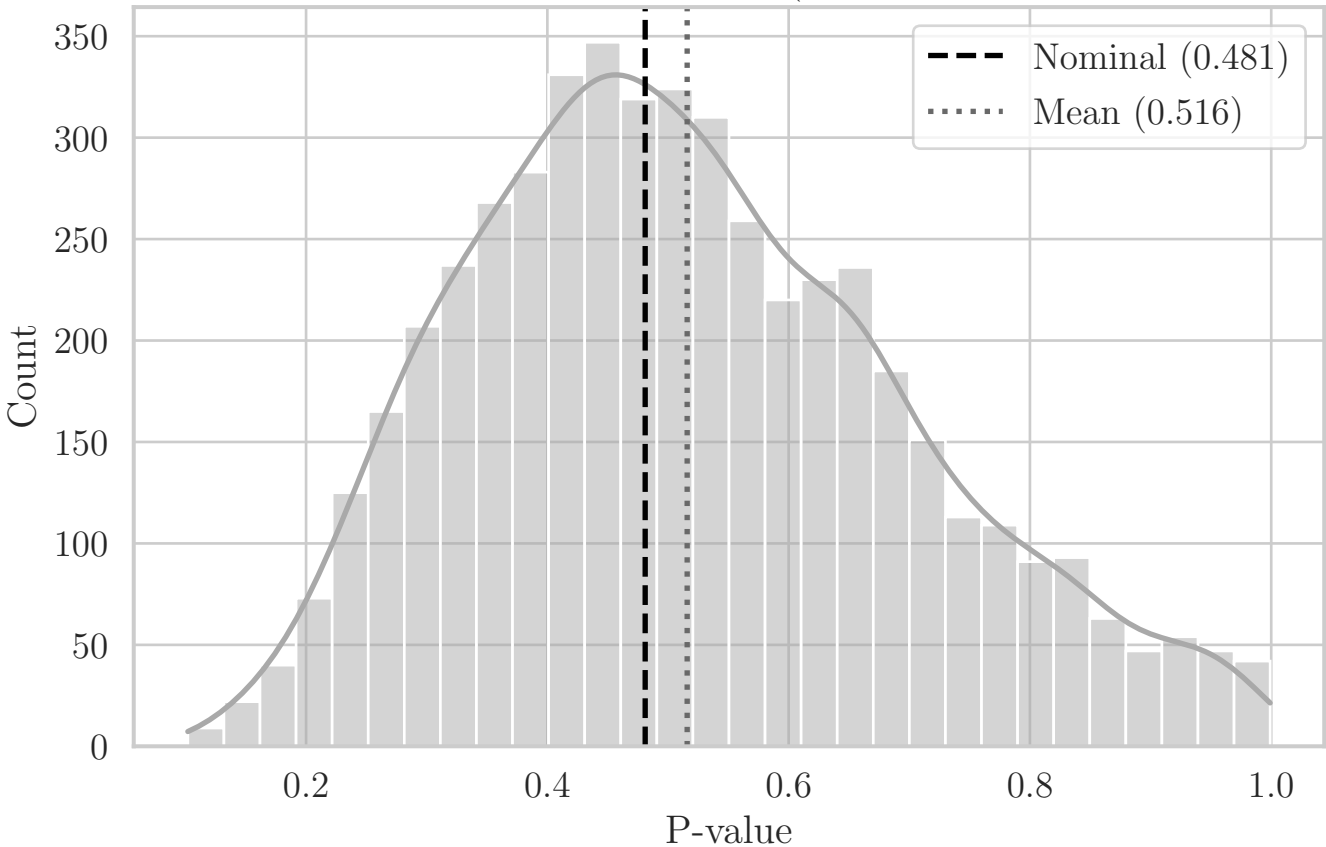
MC Distribution of P-values for QRS Angle (Aggregated Top-Right Quadrant YZ)
