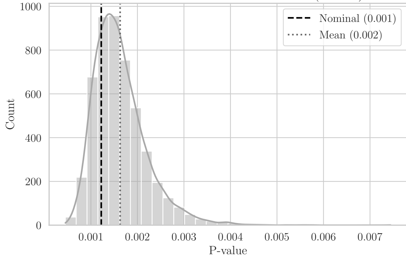
MC Distribution of P-values for T Area (YP YZ)
