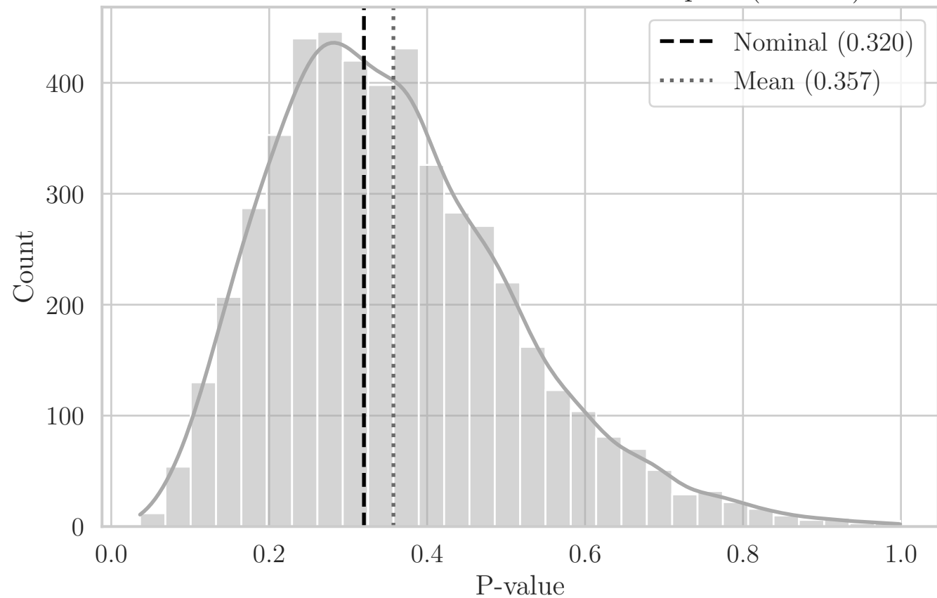
MC Distribution of P-values for T Compact (YP YZ)
