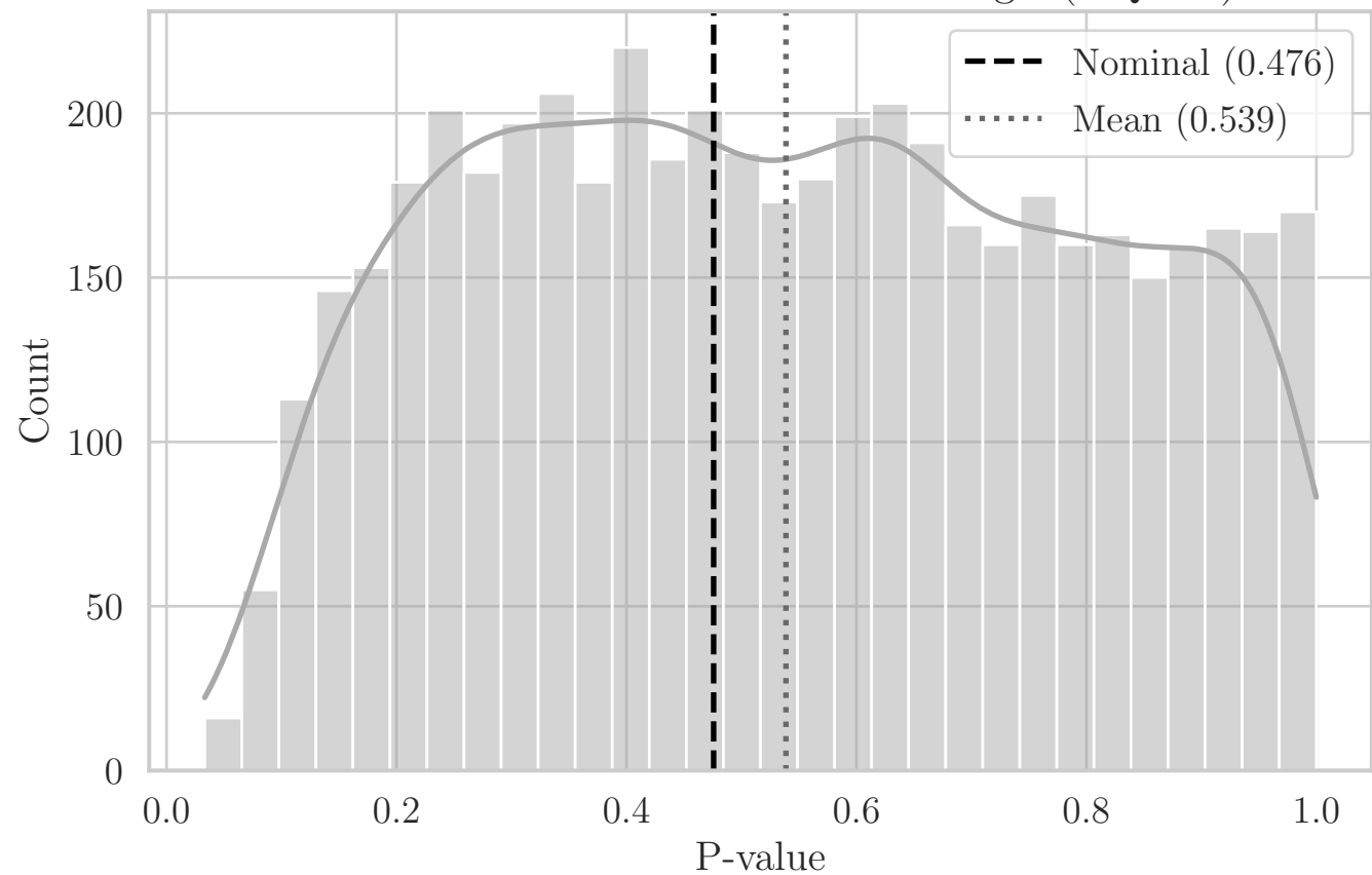
MC Distribution of P-values for T Angle (YQ XY)
