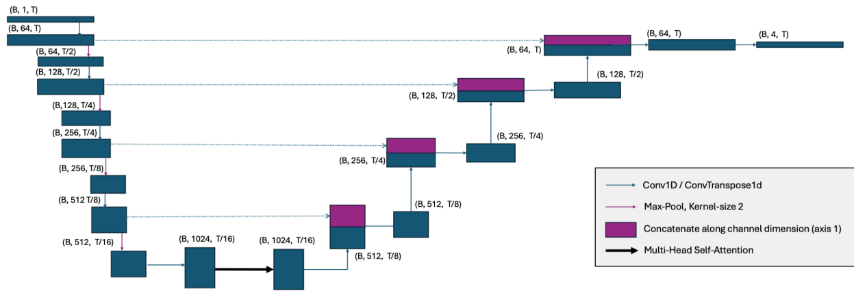
Figure 3.2 Architecture of the U-Net-1D-15M model. The diagram illustrates the data flow and tensor shape transformations, where B is the batch size (e.g., 64) and T is the number of time steps (500, corresponding to a 2-second segment). The dimensions of the blocks represent the number of channels and the temporal length, though they are not drawn to scale.
