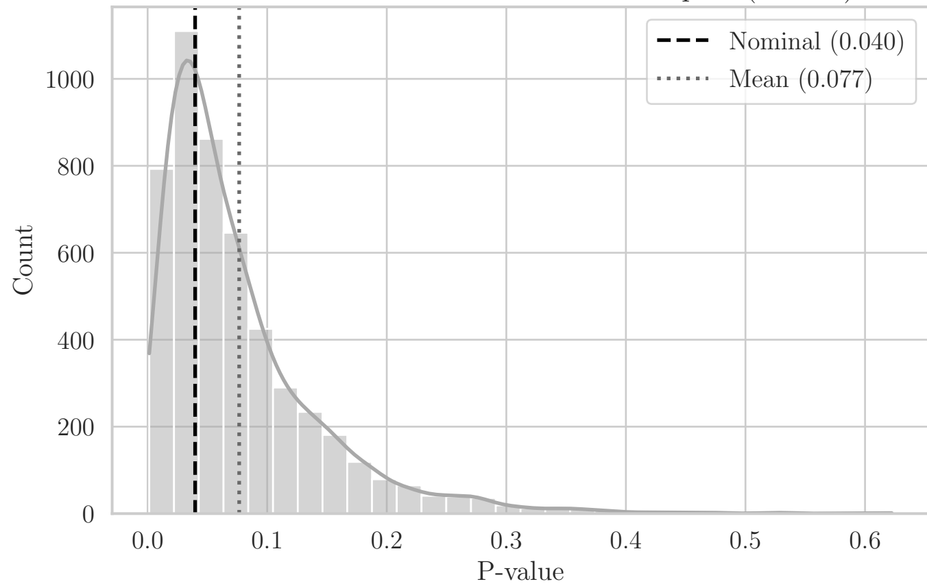
MC Distribution of P-values for T Compact (C1 XY)
