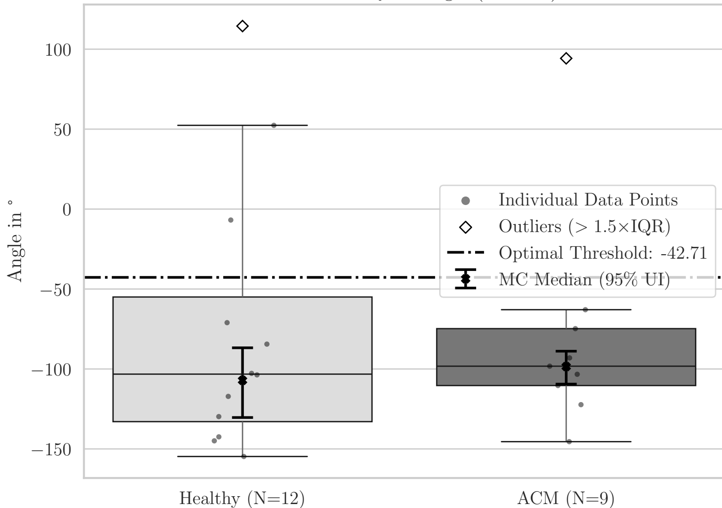
Box Plot for QRS Angle (EY XY)
