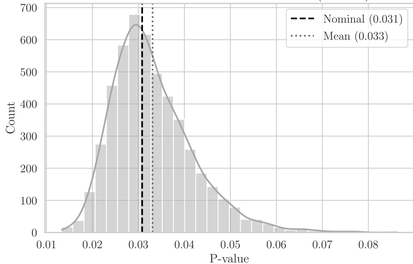
MC Distribution of P-values for T Area (OR XY)
